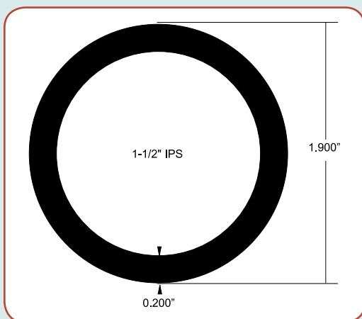
A45-8355 Aluminum Pipe
