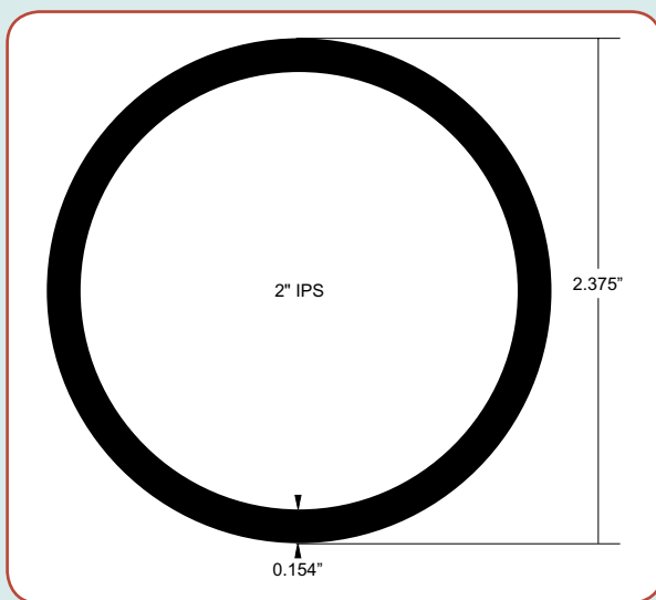
A45-0356 Aluminum Pipe
