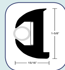
Fits V11-4014 Flexible Vinyl Rub Rail
