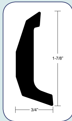
A11-0514 Aluminum Rub Rail
