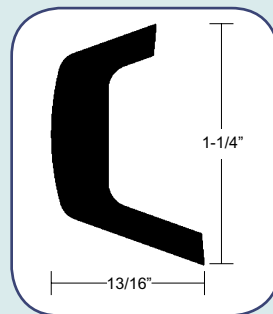
A11-0511 Aluminum Rub Rail
