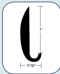
A11-0152 Aluminum Rub Rail
