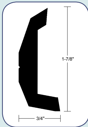
V21-3670 Rigid Rub Rail
