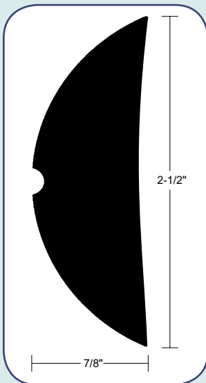
V21-0458 Rigid Rub Rail
