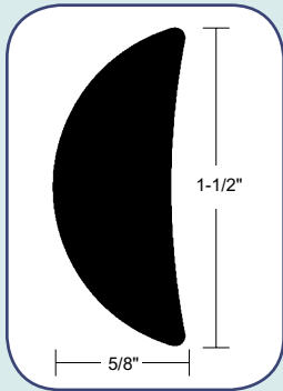
V21-0456 Rigid Rub Rail
